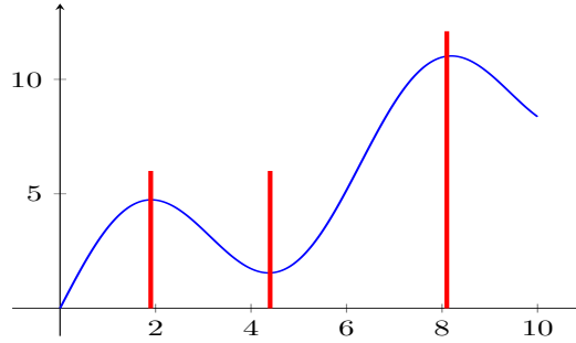
Fig. 19. Partition of the domain of a function in intervals of monotonicity.
