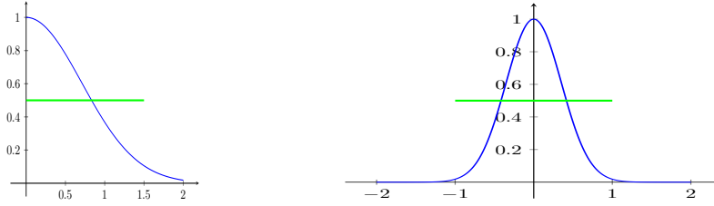
Fig. 20. Left: The monotone rearrangement u^* . Right: The symmetric rearrangement \widehat{u} .
