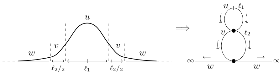
Fig. 30. How to cut a soliton to fix it on a given bubble tower.
