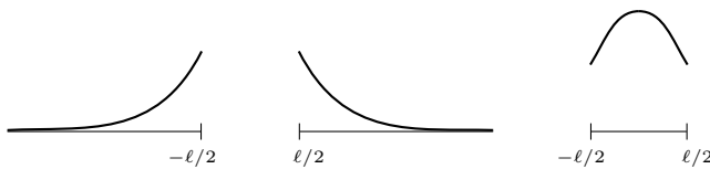
Fig. 23. One is left with one head and two tails.
