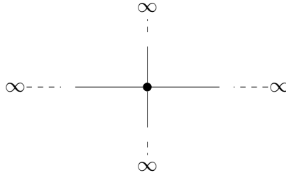
Fig. 5. A star-graph made of four halflines.
