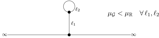
Fig. 44. A signpost graph: for every value of \ell_1, \ell_2 , this graph satisfies the hypotheses of Thm. 7.4.
