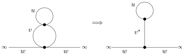
Fig. 31. From a bubble tower to a signpost.
