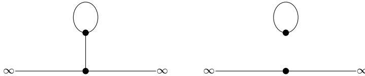
Fig. 14. Left: Signpost graph. Right: after the removal of the pendant, there remains a connected compact component made of a loop, violating (H) (see the second formulation).
