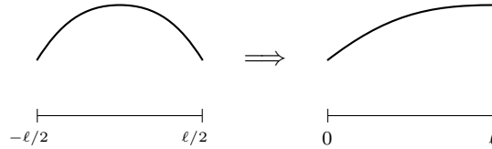
Fig. 24. Second step: glue the two tails together.
