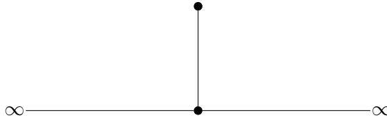
Fig. 21. A line with one pendant (bounded edge) attached to it.
