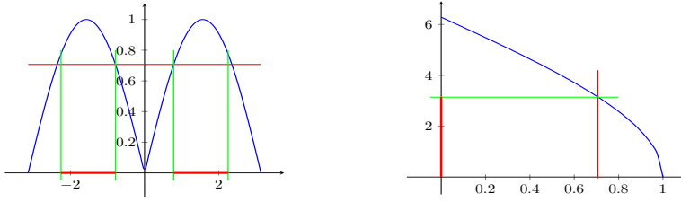
Fig. 17. Left: f(x) = |\sin x| . Right: \rho_f(t) = 2\pi - 4\arcsin x .
