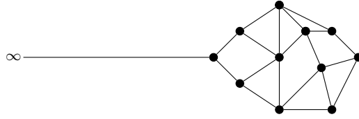
Fig. 42. Case 3: a graph with exactly one half-line.
