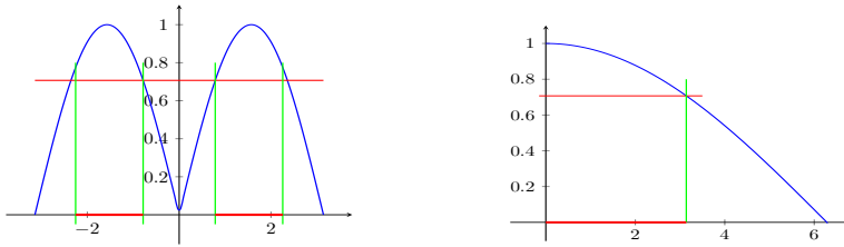
Fig. 18. Left: f(x) = |\sin(x)| . Right: f^*(x) = \cos(x/4) .
