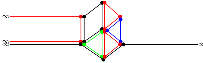
Fig. 12. A possible cycle covering.
