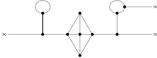
Fig. 43. Case 4: a graph without terminal points, without cycle covering and with more than one half-line. No cycle can cover the thick edge.
