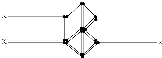
Fig. 41. The graph portrayed in Fig. 40 and a covering made of 7 cycles.
