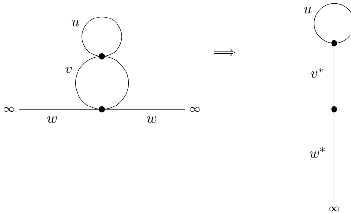
Fig. 32. From bubble tower to tadpole.
