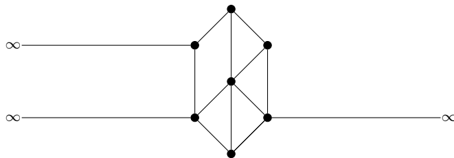
Fig. 40. Case 2: a graph satisfying assumption (H).
