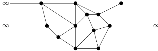
Fig. 39. Case 1: a graph with a terminal point.
