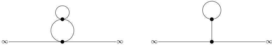
Fig. 26. Last step: mount the function on \mathcal{G} .
