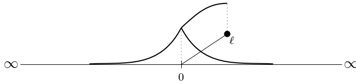
Fig. 26. Last step: mount the function on \mathcal{G} .
