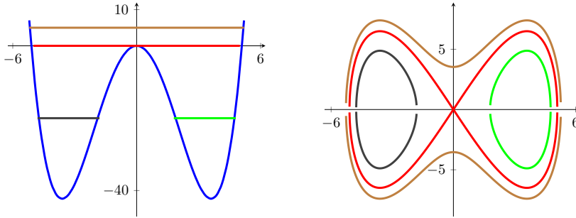
Fig. 3. Left: The profile of the potential V . Right: The phase portrait induced by the potential V .
