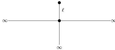
Fig. 38. A graph made of three half-lines and a terminal edge.
