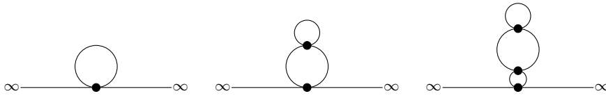
Fig. 29. Some examples of bubble towers.
