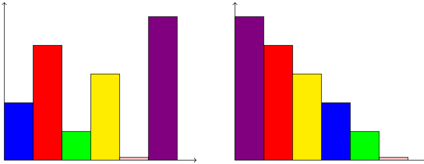
Fig. 16. Monotone rearrangement of a piecewise constant function: this example shows pictorially the fact that integral norms are preserved while oscillations are reduced, so that the nonlinear term in the energy is left untouched, while the kinetic term is dumped, so that the energy has diminished.
