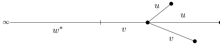
Fig. 33. Open the arcs in the bubble tower.
