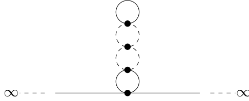
Fig. 15. A bubble tower.
